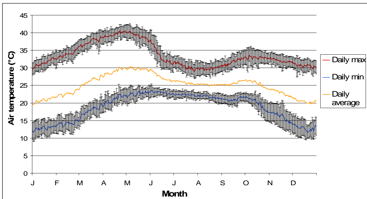
Figure 2 Temperature composite
